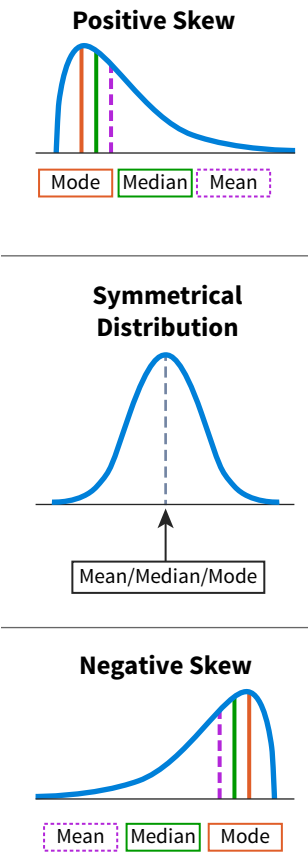
ILLUSTRATION 2.41 Skewness Examples
